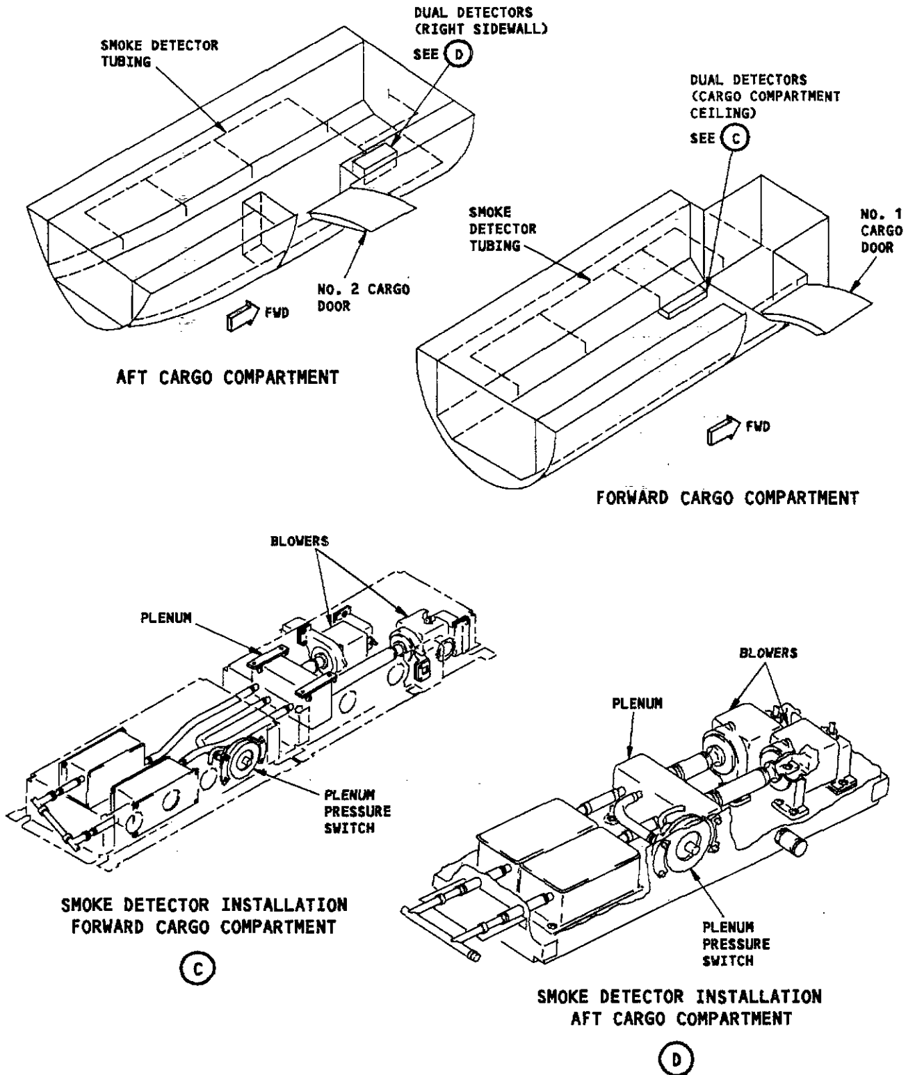
Cargo Compartment Smoke Detection System Component Location
