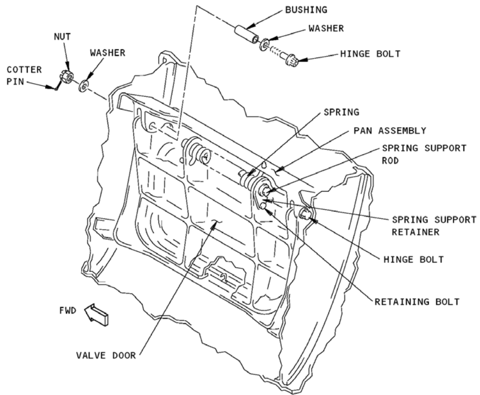
VACUUM PRESSURE RELIEF VALVE
