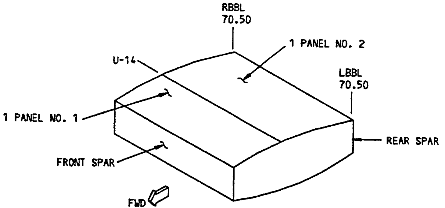
UPPER SKIN PANELS DETAIL I
