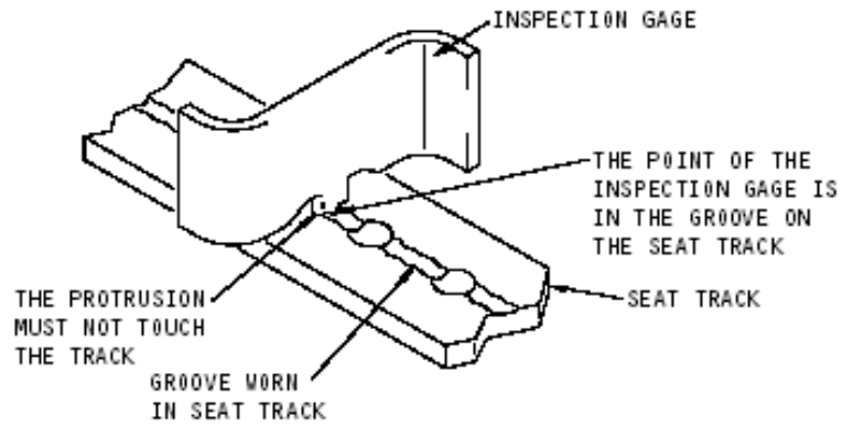
INSPECTION ON THE SURFACE OF THE SEAT TRACK
