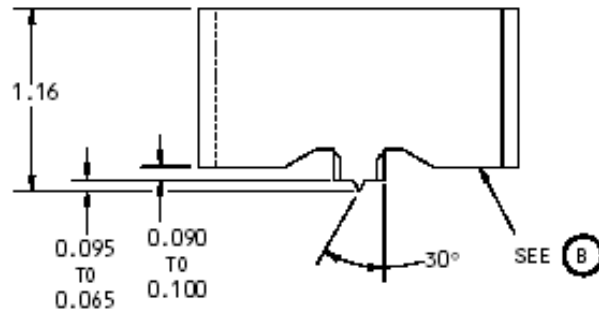
INSPECTION GAGE (SIDE VIEW)
