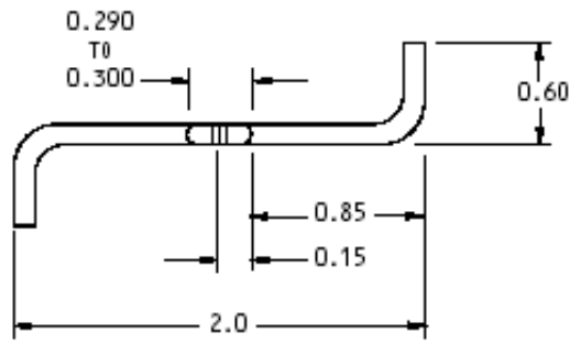
INSPECTION GAGE (BOTTOM VIEW)
