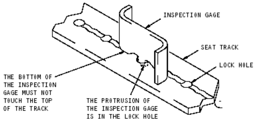
INSPECTION OF THE LOCK HOLE
