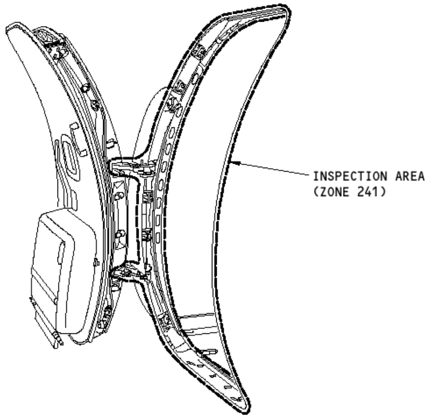
AFT ENTRY DOOR
